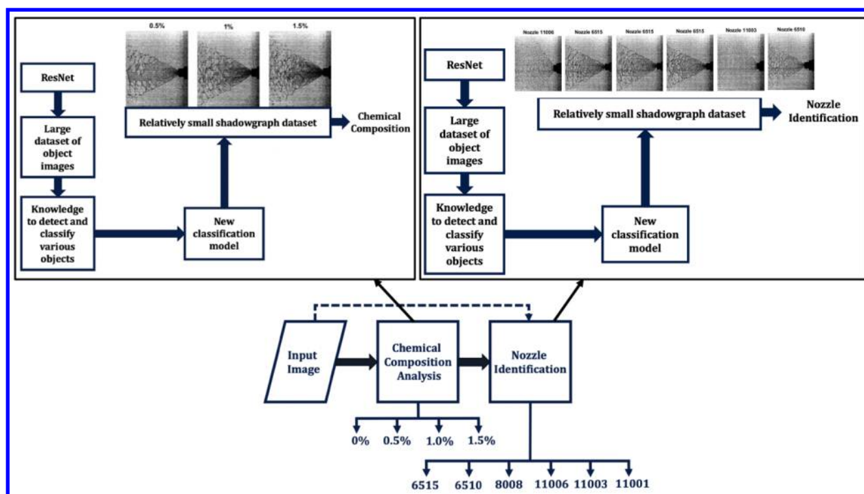
Figure 2 Machine learning architecture used to predict chemical composition and nozzle type [14]
