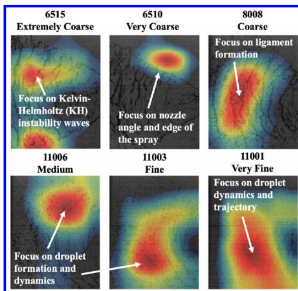
Figure 3 Mean CAM results for nozzle identification for 0% chemical composition (Water)
