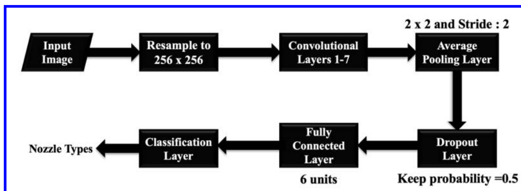
Figure 7 Block level diagram of the CNN approach used for nozzle identification from iPhone camera
