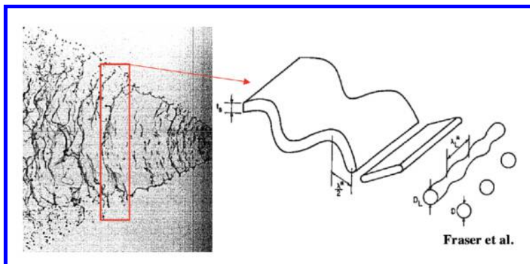
Figure 1 Shadowgraph image of the spray and the breakup mechanism proposed by Fraser et al. [8]
