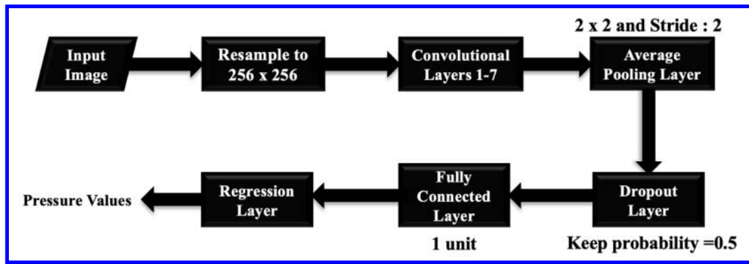
Figure 9 Block level diagram of the CNN approach used for pressure estimation on shadowgraph Images
